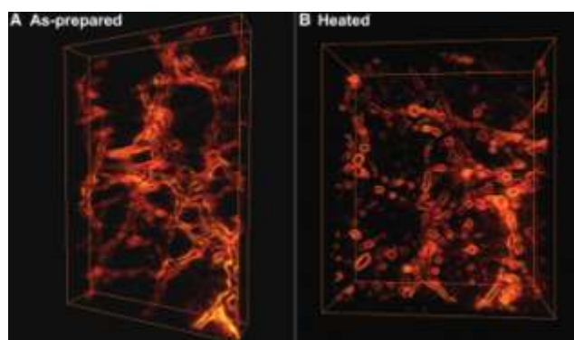
Fig. 9 Tomographic reconstructions of (a) an agarose network inside of a section of as-prepared calcite crystal and (b) cavities inside of a section of heated crystal (reproduced with permission from ref. 38)
