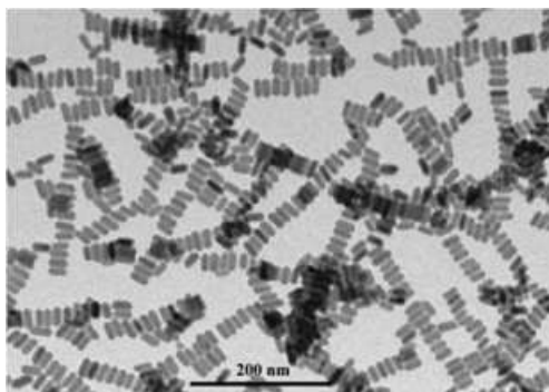
Fig. 5 TEM image showing ordered chains of prismatic \text{BaCrO}_4 nanoparticles prepared in AOT microemulsion (reproduced with permission from ref. 21)
