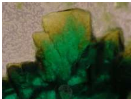
Fig. 4 Growth of yellow [\{\text{Cu}(\text{L})\}_2(\mu\text{-Cl})_3]^+ daughter phase on the green parent crystals of [\text{Cu}(\text{L})\text{Cl}_2] (reproduced with permission from ref. 20).
