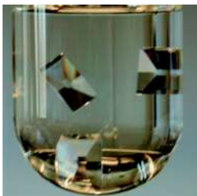
Fig. 8 asparagine monohydrate crystals with an unusual habit growing in an agarose hydrogel (reproduced with permission from ref. 35)
