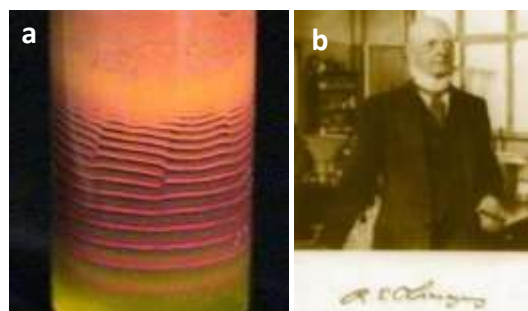
Fig. 6 (a) Liesegang rings arising from the diffusion of silver nitrate through potassium chromate in silica gel (reproduced with permission from http://polymer.bu.edu/ogaf/html/chp62exp1.htm ), (b) Raphael Eduard Liesegang
