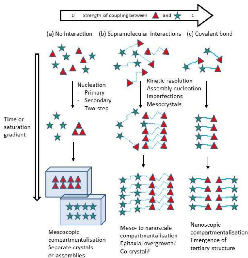
Fig. 1 Two-component, orthogonal self-assembly under a supersaturation gradient as a function of the degree of coupling between the individual components
