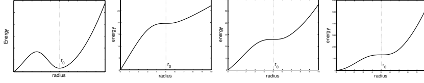
Fig. 2. Plot of E_0 against r for r_0 = 5.0 . Left: model in [1], with a local energy minimum. Right three: new model, with \alpha and \beta determined by equations (3.2). Second from left, d = 6.4 ; second from right, d = 6.8 ; far right, d = 7.2 . For this value of r_0 , d_{\min} = 6.3880 , d_{\max} = 7.2495 .
