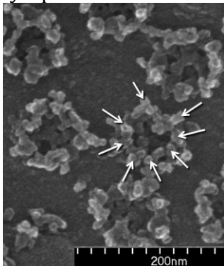
Figure 3. High resolution scanning electron microscopy of isolation Xenopus oocyte NE showing cytoplasmic filaments (arrows) where Nup358 is located.
