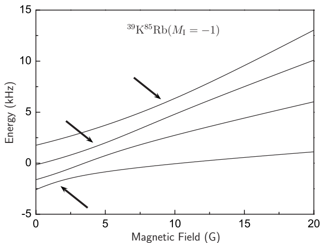
FIG. 2. Zeeman splitting and avoided crossings (indicated with arrows) for the M_I=-1 levels of ^{39}\text{K}^{85}\text{Rb}(v=0, N=0) .
