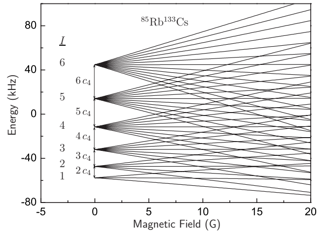
FIG. 3. Zeeman levels for ^{85}\text{Rb}^{133}\text{Cs}(v=0, N=0) .
