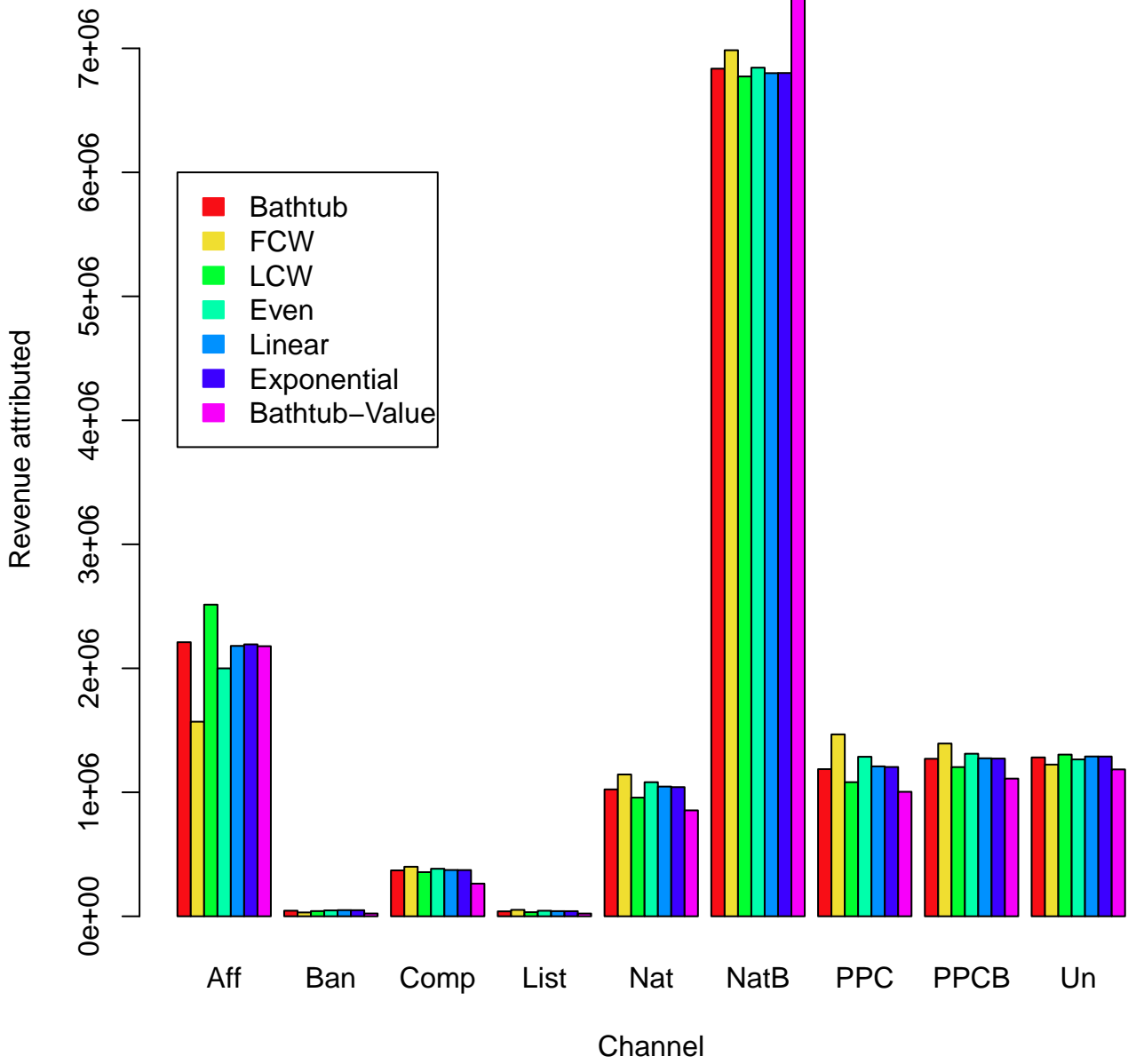
Figure 3: Comparison of total revenue attributions to eight channels for 58667 journeys for seven attribution methods.
