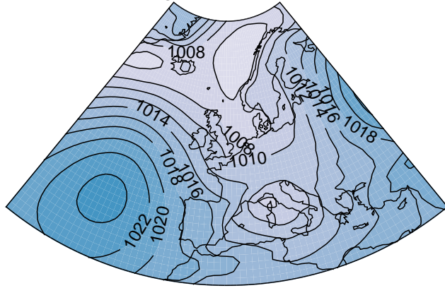
(c) Trough (TRW, TRM, TM)
