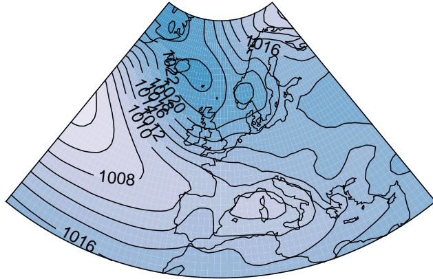
(b) Blocked (HNFZ, HNFA, HNZ, HNA)
