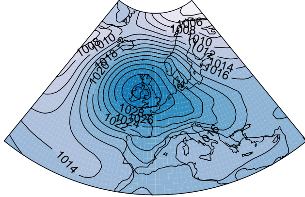
(a) High over Britain (HB)
