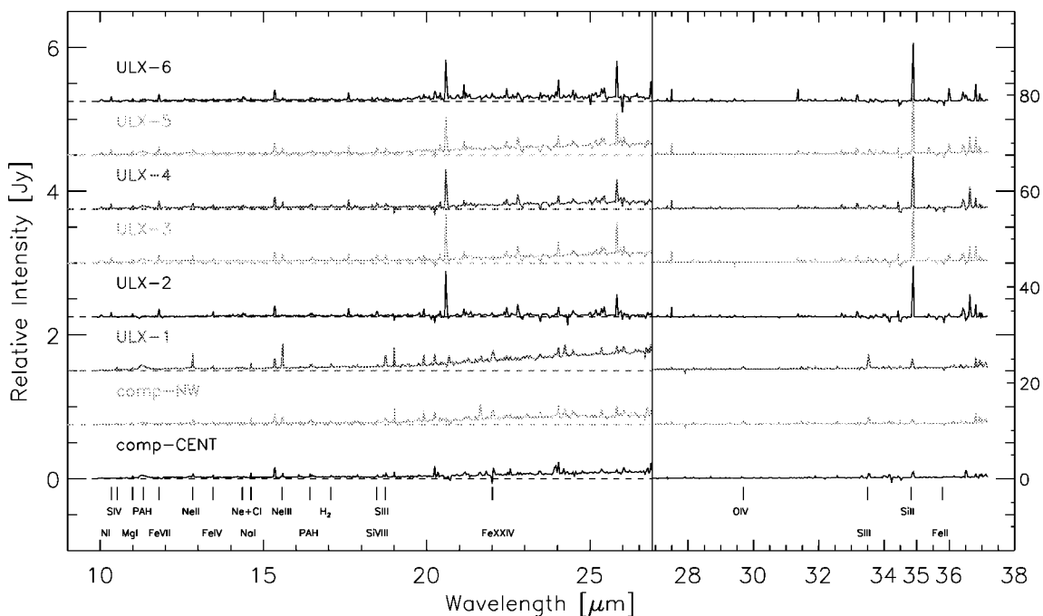
FIG. 1.—Combined spectra with the left SH and right LH modes for all of the sources analyzed in this study. For better visualization, the spectra have been plotted displaced along the y-axis. From \sim 9 to \sim 26.9 \mu\text{m} spectra are displaced by 0.75 Jy, and \sim 26.9 to \sim 38 \mu\text{m} spectra are displaced by 15 Jy. Dashed lines are set to help indicate the slope of the continuum at wavelengths \geq 20 \mu\text{m} . [See the electronic edition of the Journal for a color version of this figure.]
