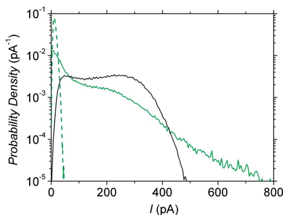
Fig. 3 c-AFM current distribution profiles for pristine P3HT ( p = 1 ) (black solid), p = 0.37 a-PS:P3HT blend (green dash) and p = 0.41 i-PS:P3HT blend (green solid).
