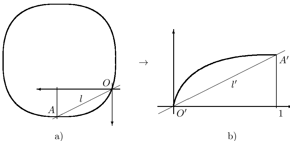
Figure 1: Geometric construction of the Wulff profile
