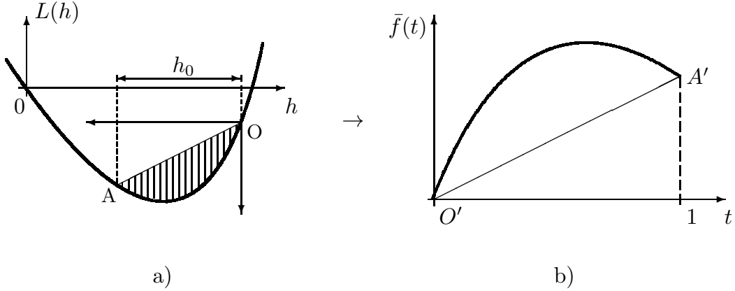
Figure 2: Wulff construction in a general 1D model of SOS type
