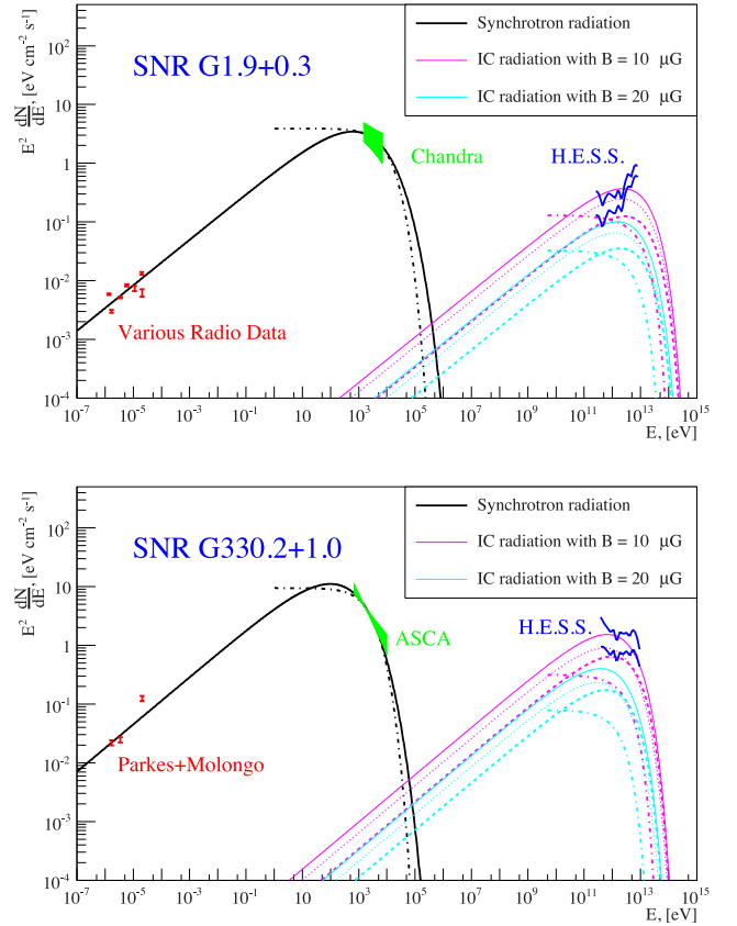
Figure 2. SEDs of G1.9+0.3 (top) and G330.2+1.0 (bottom) in a leptonic scenario. The H.E.S.S. ULs on the differential flux are shown assuming two different spectral indices, 2.0 (lower curve) and 3.0 (upper curve). The multifrequency radio data shown for G1.9+0.3 was compiled by Green et al. (2008); additional ULs in the IR domain (Arendt 1989) are not shown because they lie outside of the plotted range and are not constraining. The solid and dot-dashed lines represent the modelled synchrotron and IC emission spectra from uncooled and cooled (due to synchrotron losses) electron spectrum, respectively. For the IC emission, dotted (resp. dashed) lines correspond to the contribution due to IC scattering on CMB (resp. IR) photons, in the case of the uncooled electron spectrum. The IC emission is calculated for two assumptions on B . Note that the lower limit on the magnetic field is calculated comparing the integral UL on the \gamma -ray flux above the safe energy threshold to the model prediction of the flux above the same energy. See Section 4.1 for details. (A colour version of this figure is available in the online journal.)
