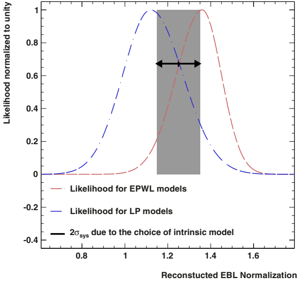
Fig. A.2. Likelihood profiles as a function of the normalized EBL opacity. The profiles were normalized to unity for clarity purposes. The dot-dashed curve is derived fitting log-parabolic intrinsic spectra to the data sets, while the dashed curve is derived by fitting exponential cut-off models. The gap between the two profiles due to the intrinsic spectral modelling is represented by the grey shaded area and the double arrow.
