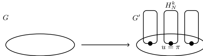
Fig. 3. The graph G' formed by attaching G to copies of H_N^k .
