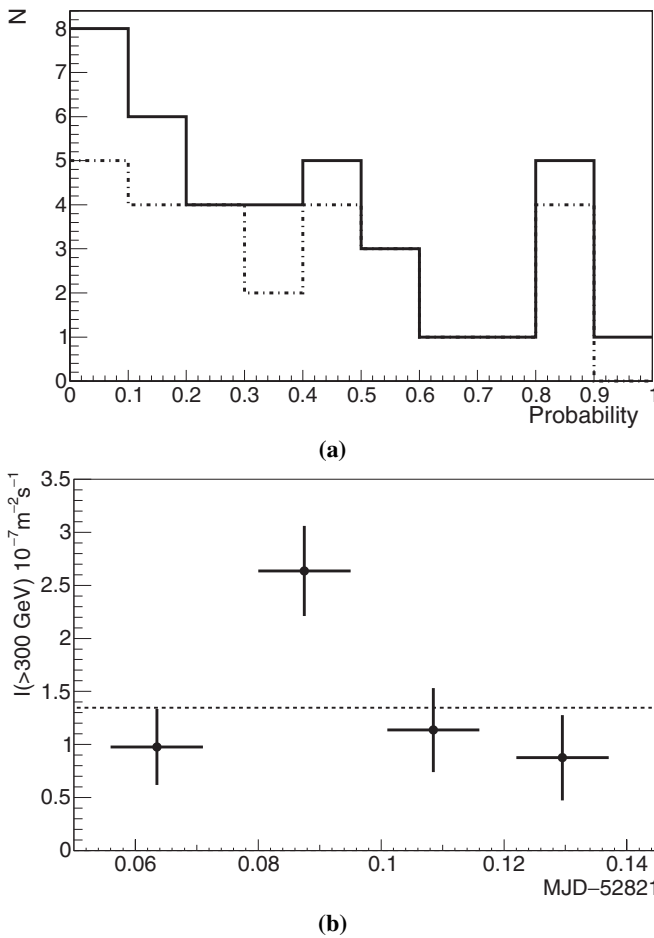
Fig. 8. a) The distribution of \chi^2 probabilities from best fits to a constant of the run by run integral flux greater than 300 GeV for each night of H.E.S.S. observations of PKS2155–304 in 2003. The solid line is for all nights of data taking and the dashed line represents nights with more than one degree of freedom (3 runs minimum). b) The run by run integral flux greater than 300 GeV observed from PKS 2155–304 for the night of MJD 52821. Only the statistical errors are shown.
