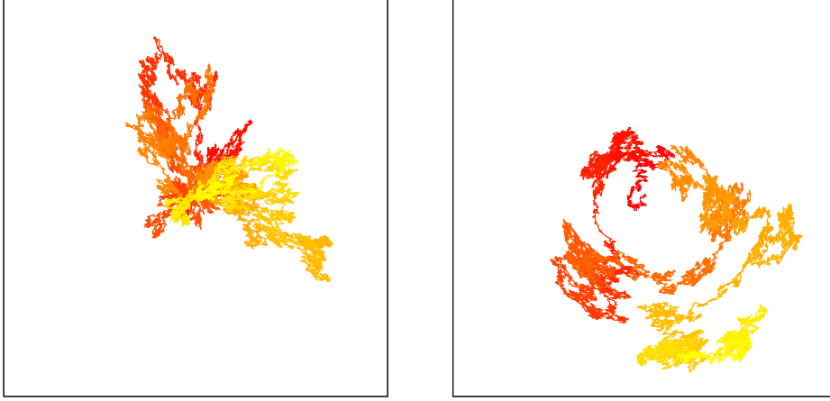
FIGURE 4: Simulation of the elliptic random walk in \mathbb{R}^2 for the recurrent case a > b (left) and the transient case a < b (right).
