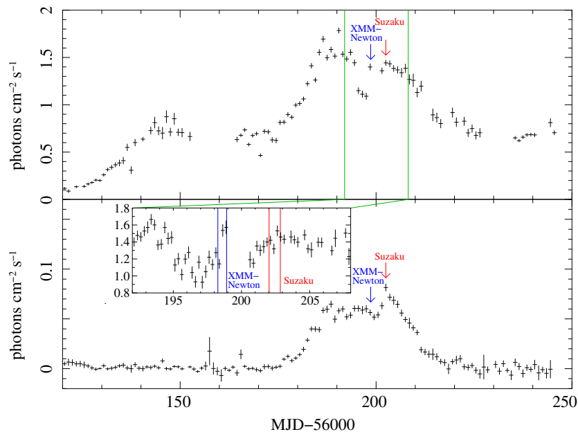
Figure 1. Long-term light curves of 4U 1630–47 in the 3–10 keV and 15–50 keV bands obtained with the Monitor of All-Sky X-ray Image /Gas Slit Camera ( MAXI /GSC) (top panel) and Swift /BAT (bottom panel), respectively.
