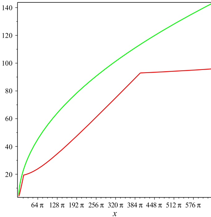
Fig. 2 The graphs of the function from Proposition 3.3 (green) and the functions from [2] (red) in the case of \alpha = (\sqrt{21} + 3)/6 = [1; 3, 1, 3, \dots] . In this case we take q_N = 4 , \lambda_N = (\sqrt{21} - 3)/2 and t = 1 . (Compare Figure 3 of [2]). (Color figure online)
