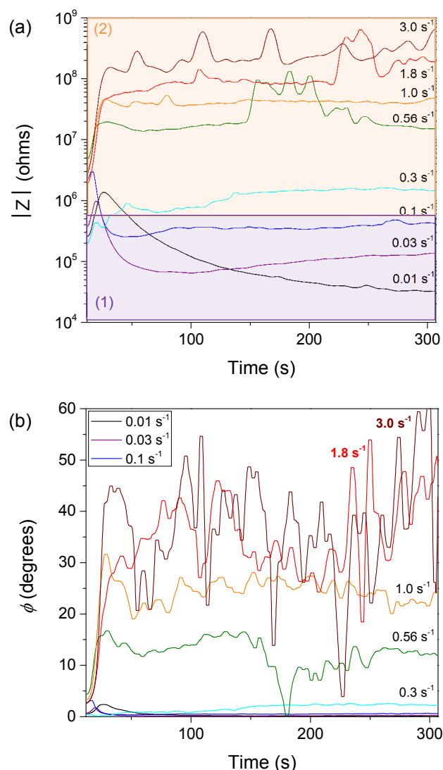
Figure 3. Polystyrene + 5 vol. % GNPs during shear: (a) Change in the impedance, |Z| , during shear at rates of 0.01 - 3 \text{ s}^{-1} , (b) Change in the phase angle of the impedance, \phi , during shear. Different stages in the processing are highlighted in (a), corresponding to the steps in Figure 1. The relative contributions of the resistance and reactance of the network are shown in Supporting Information Figure S7.
