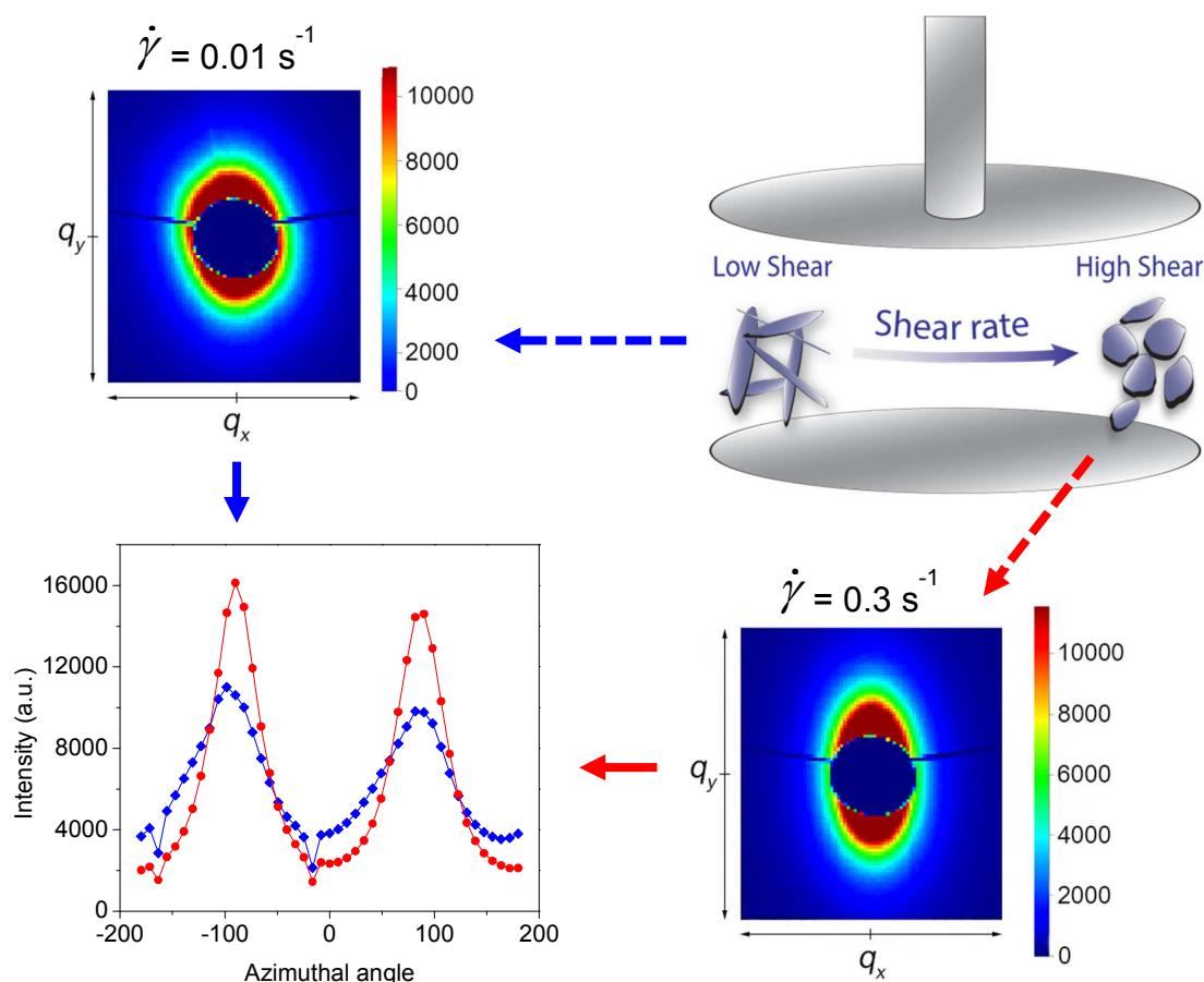
Figure 6: SAXS of polystyrene + 5 vol. % GNPs composites at 200 °C; 2D scattering patterns following 0.01 \text{ s}^{-1} shear and 70 s of 0.3 \text{ s}^{-1} shear. Anisotropy in the scattering pattern shows the alignment of the GNPs in the composite, which increases following the increased shear. The scattering intensity as a function of the azimuthal angle in the q range 0.002\text{-}0.0035 \text{ \AA}^{-1} is plotted. Samples following 0.01 \text{ s}^{-1} ( \blacklozenge ) and 0.3 \text{ s}^{-1} ( \bullet ) shear are shown, calculated from the 2D scattering patterns. Zero degrees represents the 3 o'clock position on the detector image and the angle increases in the clockwise direction. The orientation factor increases from 0.27 to 0.47 between these shear rates.
