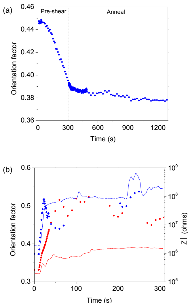
Figure 7. Orientation factors calculated for composites of polystyrene + 5 vol. % GNPs from SAXS under shear at 200^\circ\text{C} . (a) Orientation factor of GNPs during a pre-shear at a rate of 0.01 \text{ s}^{-1} and subsequent annealing step. (b) Orientation factors (symbols) and impedance |Z| (lines) during shear at rates of 0.3 (●—) and 1.8 \text{ s}^{-1} (◆—).
