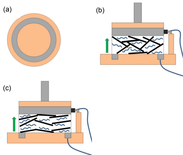
Figure 2. Schematic of the rheo-impedance device: (a) A ring electrode acts as the bottom plate, giving a well-defined shear rate for the measurements, (b) A well-developed GNP network structure giving a low impedance, (c) Aligned GNPs give a high impedance
