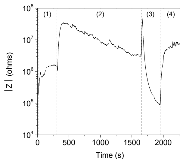
Figure 5. Impedance, |Z| , of polystyrene + 5 vol. % GNPs during cyclic processing at 200^\circ\text{C} during (1) 0.3 \text{ s}^{-1} shear, (2) annealing, (3) 0.01 \text{ s}^{-1} shear and (4) annealing.
