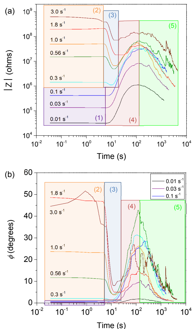
Figure 4. Polystyrene + 5 vol. % GNPs during annealing at 200 \text{ }^\circ\text{C} : (a) Change in the impedance, |Z| , and (b) the phase angle of the impedance, \Phi , following cessation of shear as a function of the preceding shear rate. Different stages in the processing are highlighted in (a) and (b), corresponding to the steps in Figure 1.
