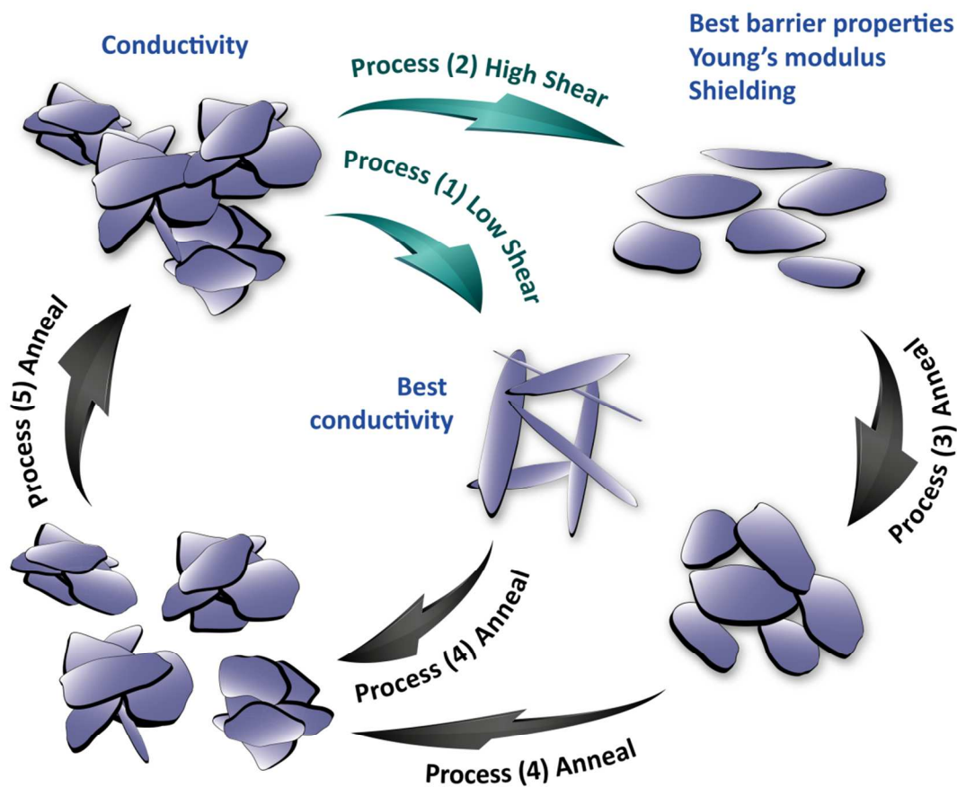
Figure 1. Schematic of processing effects on the GNP structure within the composite: Initially the composite has an agglomerated structure that has formed a network. Under low shear (1) this can break apart the agglomerates and exfoliate graphene, forming a more effective network, enhancing the conductivity. At higher shear rates (2) the conductivity reduces with increasing alignment of the GNPs. During annealing the aligned GNPs begin to relax, increasing the conductivity (3), but with more annealing the GNPs will re-agglomerate into discrete agglomerates of GNPs, decreasing the conductivity (4). Eventually a secondary agglomeration of the GNPs occurs, forming a connected network, and enhancing the conductivity again (5). The best processing steps for particular properties are highlighted.
