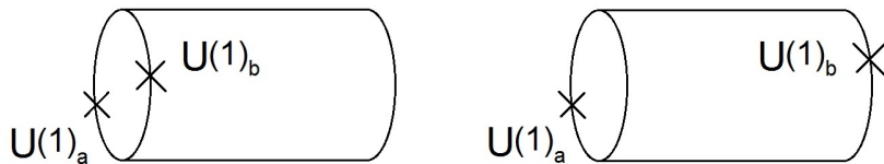
Figure 4: String diagrams contributing to kinetic mixing of U(1) s defined across multiple orbifold fixed points.
