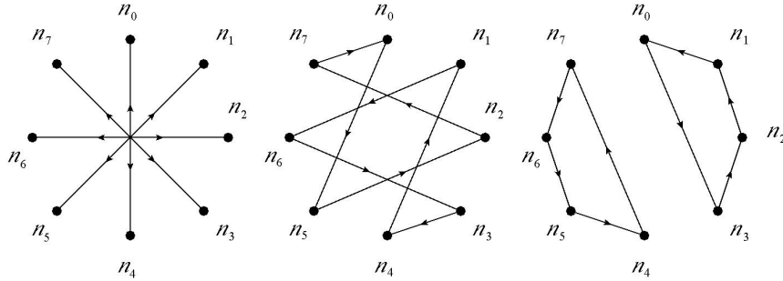
Figure 9: Quiver for the \mathbb{Z}_2 \times \mathbb{Z}_4 orbifold singularity. For better visualisation the quiver is split into three diagrams. The diagrams show the matter content that is allowed by the orbifold twists \{\theta_1, \eta_1\} , \{\theta_2, \eta_2\} and \{\theta_3, \eta_3\} respectively.
