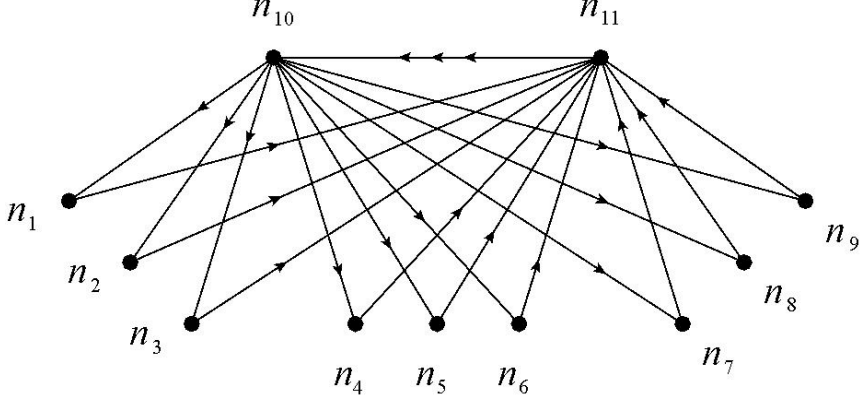
Figure 7: The quiver for the \Delta_{27} singularity
