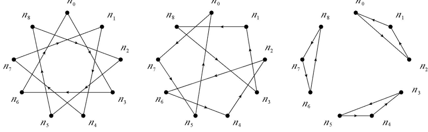
Figure 10: Quiver for the \mathbb{Z}_3 \times \mathbb{Z}_3 orbifold singularity. For better visualisation the quiver is split into three diagrams. The diagrams show the matter content that is allowed by the orbifold twists \{\theta_1, \eta_1\} , \{\theta_2, \eta_2\} and \{\theta_3, \eta_3\} respectively.
