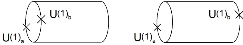
Figure 3: String diagrams that contribute to mixing between two U(1) s labelled by a and b at \mathcal{O}(B^2) .
