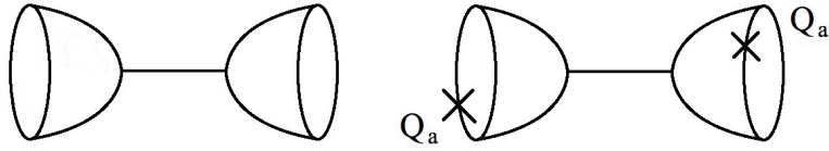
Figure 2: The annulus string diagram in the open string UV/ closed string IR limit l = 1/t \rightarrow \infty . Both ends of the left diagram are proportional to tadpoles. The right diagram has insertions of a U(1) generator on both its boundaries and is used to calculate Green-Schwarz couplings which give a mass to U(1) gauge bosons.
