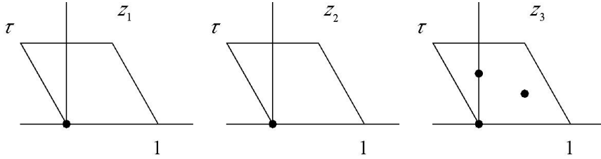
Figure 5: The \mathbb{T}^6/\mathbb{Z}_6 orbifold. Dark circles correspond to fixed points under all orbifold twists and \tau is the complex modulus of the tori.
