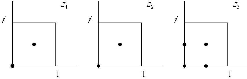
Figure 1: The \mathbb{T}^6/\mathbb{Z}_4 orbifold. The circles indicate the positions of the 16 orbifold fixed points.
