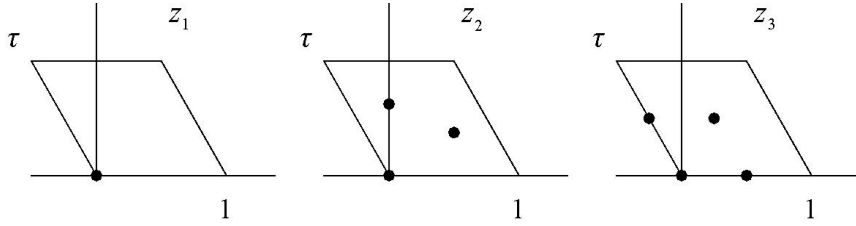
Figure 6: The \mathbb{T}^6/\mathbb{Z}'_6 orbifold. Dark circles correspond to fixed points under all orbifold twists and \tau is the complex modulus of the tori.
