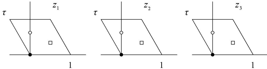
Figure 8: The \mathbb{T}^6/\Delta_{27} orbifold. The filled circle, the hollow circle and the square denote the coordinates of the three fixed points in the compact space.
