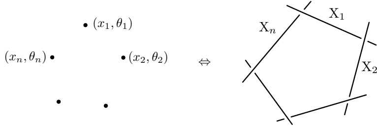
Figure 2: The n generic points (x, \theta) correspond to n lines ( \mathbb{C}\mathbb{P}^1 s) in \mathbb{C}\mathbb{P}^{3|4} . In the limit that (x_i - x_{i+1}) \rightarrow \tilde{\lambda}_i \lambda_i and (\theta_i - \theta_{i+1}) \rightarrow \eta_i \lambda_i , these lines intersect in supertwistor space, forming a nodal curve C .
