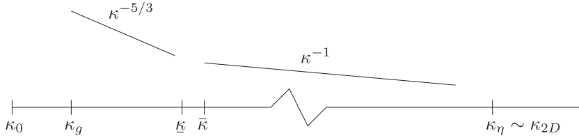
FIG. 2. Expected tracer spectra for the case of inverse cascade with a moderate Schmidt number.
