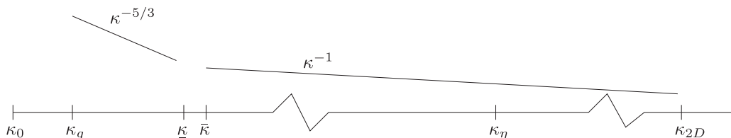
FIG. 1. Expected tracer spectra for the case of inverse cascade with a large Schmidt number.
