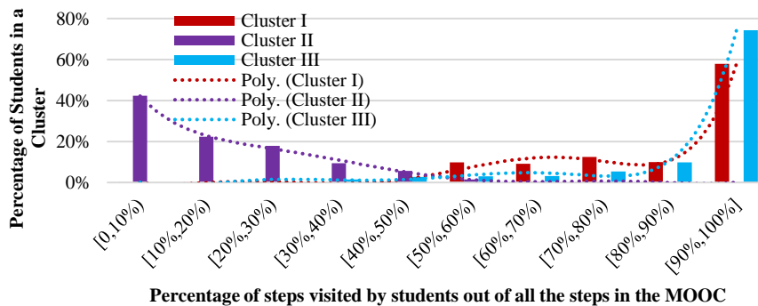
Fig. 4. Comparison of the number of steps visited by students between three clusters
