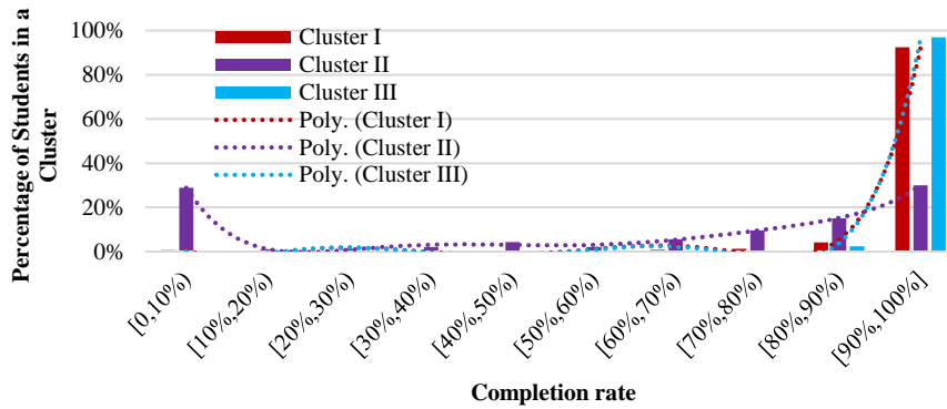
Fig. 5. Comparison of completion rate between three clusters
