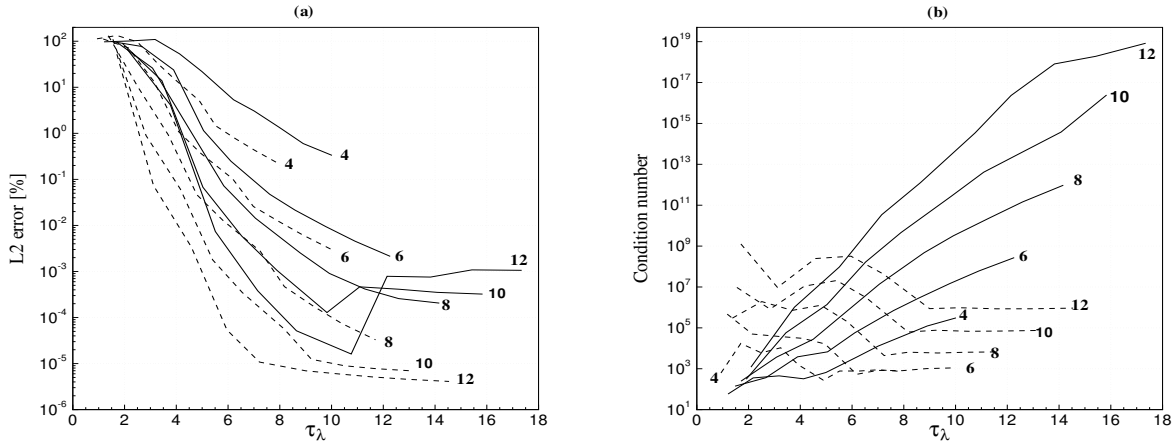
Figure 11: The L^2 error (left) and condition number (right) against \tau_\lambda ; ka = 25\pi . Solid lines (PUFEM), dashed lines (BBFEMs).
