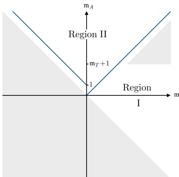
Figure 6. Summary of the structure of the moduli space and supersymmetric ground states in the (\mathbf{m}, \mathbf{m}_A) plane. There are no supersymmetric ground states in the shaded regions.
