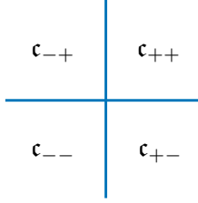
Figure 3. Chambers in the space of real mass parameters (m_1, m_2) \in \mathfrak{t}_f = \mathbb{R}^2 for two chiral multiplets \phi_1, \phi_2 and Fermi multiplet with superpotential J = \phi_1\phi_2 .
