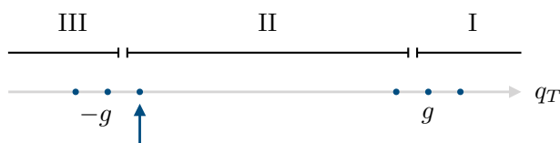
Figure 4. We separate our discussion of the supersymmetric ground states for the XYZ model into three regions depending on the U(1)_T flavour symmetry charge q_T . An arrow marks the point in region II where we obtain a complete result.
