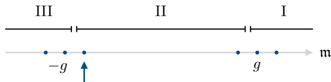
Figure 5. We separate our computation of the supersymmetric vacua for supersymmetric QED into three different regions depending on the flux \mathbf{m} \in \mathbb{Z} . An arrow marks point in region II discussed in the main text.
