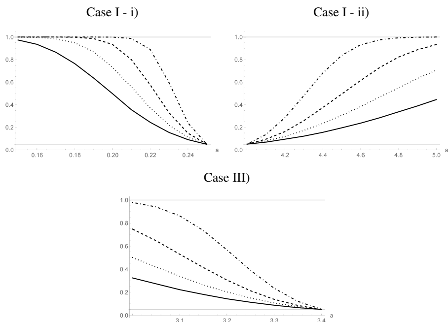
Figure 4: Power plots for different sample sizes. n = 50 (solid line), n = 100 (dotted line), n = 200 (dashed line) and n = 500 (dotted-dashed line)
