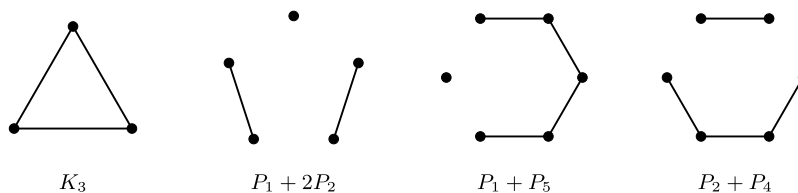
Fig. 1. The forbidden induced subgraphs considered in our results.
