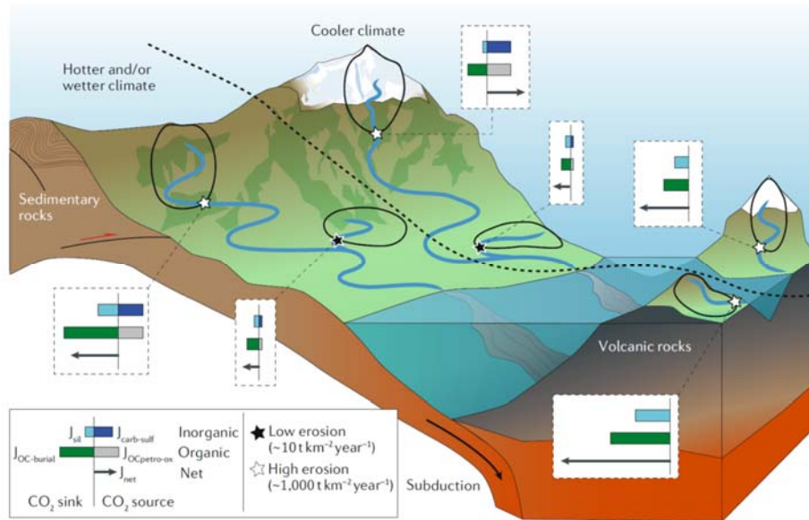
1490 Figure 5: A new view of mountains, erosion and the carbon cycle. Schematic of the CO 2 1491 sources and sinks by weathering in different environments, including fluxes in the inorganic 1492 carbon cycle ( J_{\text{sil}} = silicate weathering, light blue; J_{\text{carb-sulf}} = sulfide oxidation, dark blue) and 1493 organic carbon cycle ( J_{\text{OCburial}} = OC burial, dark green; J_{\text{OCpetro-ox}} = rock organic carbon 1494 oxidation, grey), along with the net effect of “rock-atmosphere” fluxes on CO 2 (black arrow). 1495 The cartoon considers catchments with high erosion rates, where reactions may be 1496 “kinetically limited”, and low erosion rates, where reactions are “supply limited”, shown by 1497 the white and black stars, respectively. The influence of lithology is shown by sedimentary 1498 rock-dominated catchments on the left side, and catchments underlain by volcanic rocks on 1499 the right. The dotted line separates: a) hotter or wetter climates on the near side; and b) cooler 1500 climates on the on the far side. Stylized fluxes represent qualitative estimates from these 1501 different environments based on data collected to date (Fig. 4).
