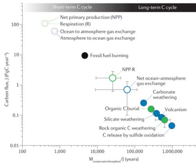
1439 Figure 2: Comparison of major fluxes and timescales of relevance in the global carbon 1440 cycle. Estimated pre-industrial fluxes of carbon (J) (refs. 48, 49 ) are shown along with the 1441 timescale required for each flux to replace the entire carbon mass of the oceans, atmosphere 1442 and biosphere ( M_{\text{ocean+atm+biosphere}} = 43,540 \pm 550 \text{ PgC} ). Green symbols denote the organic 1443 carbon cycle, and blue the inorganic carbon cycle. Open circles show processes that dominate 1444 the ‘short-term’ carbon cycle (<100,000 years), which include net primary production on land 1445 and in the ocean, respiration, and ocean-atmosphere gas exchanges. The net difference 1446 between the short-term fluxes (“NPP – R”, and “Net ocean-atmosphere gas exchange”) can 1447 control the carbon cycle over decades to thousands of years. The processes that dominate the 1448 long-term carbon cycle, over 10^5 to 10^6 year timescales, are shown as filled circles. The rapid 1449 acceleration of rock organic carbon oxidation by fossil fuel burning is highlighted as a black 1450 symbol.
