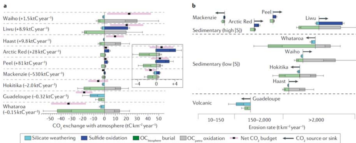
Figure 4: Net “rock-atmosphere” CO 2 exchange in river catchments. A. The potential CO 2 sinks by silicate weathering (light blue) and biospheric organic carbon (OC biosphere ) burial (green) are shown as negative fluxes. CO 2 sources via oxidative weathering of rock-derived organic carbon (OC petro ; grey) and sulfides (dark blue) are shown as positive fluxes. Uncertainties on all fluxes are provided as whiskers. The net geochemical carbon flux in each catchment is given as a black tick (uncertainty range provided by pink bars). Numbers in parentheses beside catchment names represent the net transfer of CO 2 in ktC yr -1 . Inset shows magnification of catchments with lower yields. B. CO 2 sources and sinks shown by the same coloured bars as in part A, but the catchments are arranged in terms of lithology and physical erosion rate. The black arrow indicates whether the net CO 2 exchange is a source or sink (refer to part A for the absolute values). Compiled data 41-43,69,93,139-145 are provided in the Supplementary Information.
