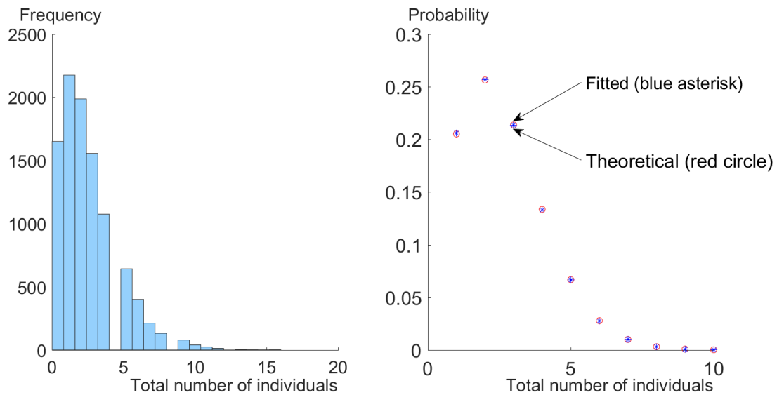
Figure 3: \beta = 0 , \mu = 0.2 , \gamma = 0.5 , \kappa = 1 . The left panel is the histogram for N(\infty, -5) ; the right panel shows that the distribution fitted for the histogram is close to the theoretical distribution for N(\infty, -5) .
