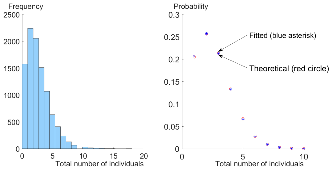
Figure 2: \beta = 0 , \mu = 0.2 , \gamma = 0.5 , \kappa = 1 . The left panel is the histogram for N(\infty, 4) ; the right panel shows that the distribution fitted for the histogram is close to the theoretical distribution for N(\infty, 4) .
