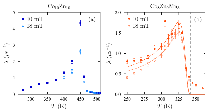
FIG. 4. Extracted values of \lambda from fitting LF \mu\text{SR} measurements of (a) \text{Co}_{10}\text{Zn}_{10} and (b) \text{Co}_8\text{Zn}_9\text{Mn}_3 . The dashed lines indicate the average value of T_c in each sample according to the relaxing amplitude. Fits in (b) are described in the main text.
