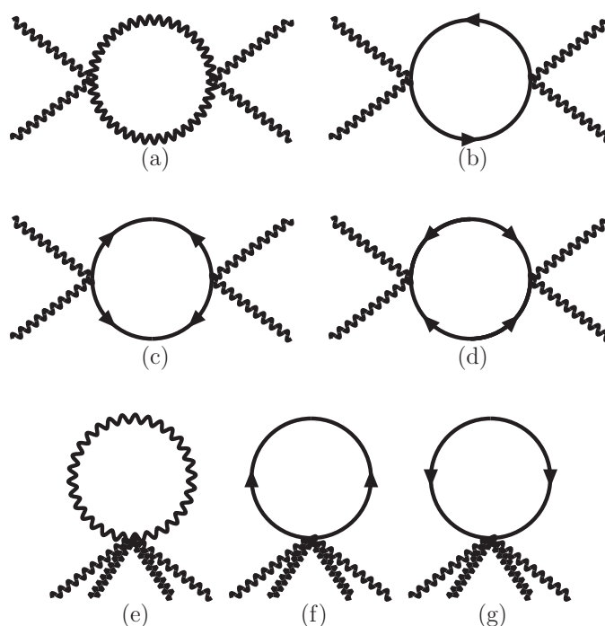
Figure 7. The s -channel one-loop scattering of \sigma\sigma \rightarrow \sigma\sigma . The one-loop scattering of \phi\phi \rightarrow \phi\phi scatterings diagrams are identical. t - and u -channels are obtained via symmetry crossing. The divergences from the fermion loops are cancelled by the “octopus” diagrams, as required by supersymmetry.
