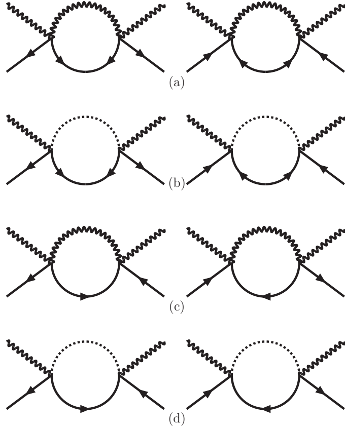
Figure 8. The scattering \sigma F_{s_2} \rightarrow \sigma F_{s_4} to one-loop order. The one-loop scattering diagrams of \phi F_{s_2} \rightarrow \phi F_{s_4} are identical. There are also two “octopus” diagrams (not shown) that cancel each other.
