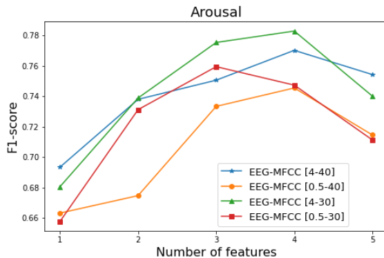
Figure 2: F1-score as a function of the number of features used to build the arousal model.
