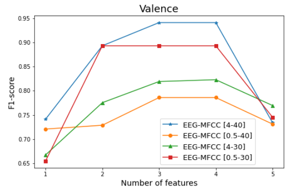
Figure 1: F1-score as a function of the number of features used to build the valence model.
