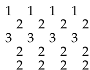
Figure 4: Frieze of type D_4 .
