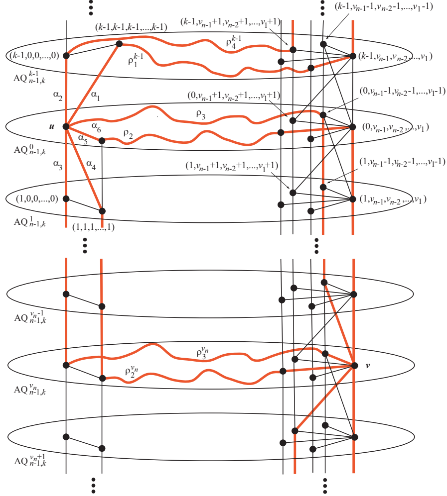
Figure 3. The 6 disjoint paths in Sub-case 2.1.
