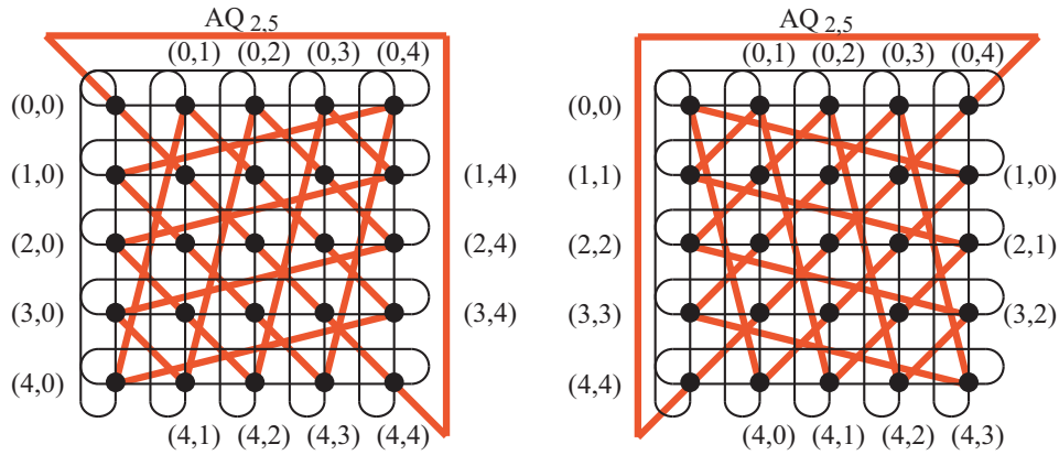
Figure 1. Two views of an augmented 5-ary 2-cube.
