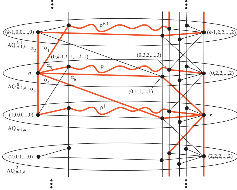
Figure 7. The paths in Sub-case 3.2.
