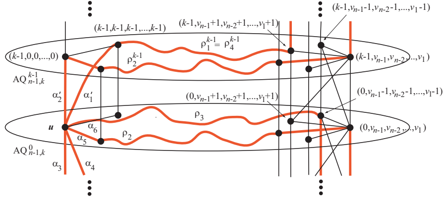
Figure 4. The amendments in Sub-case 2.2.
