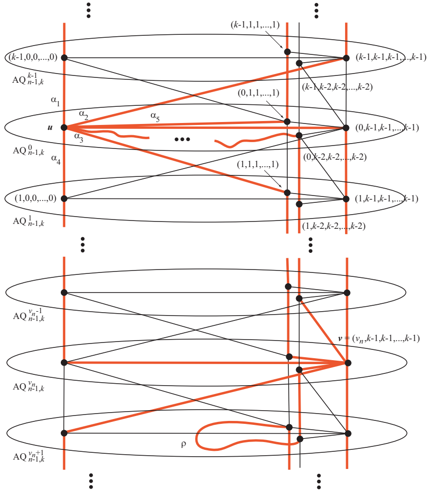
Figure 10. The paths in Sub-case 4.3.
