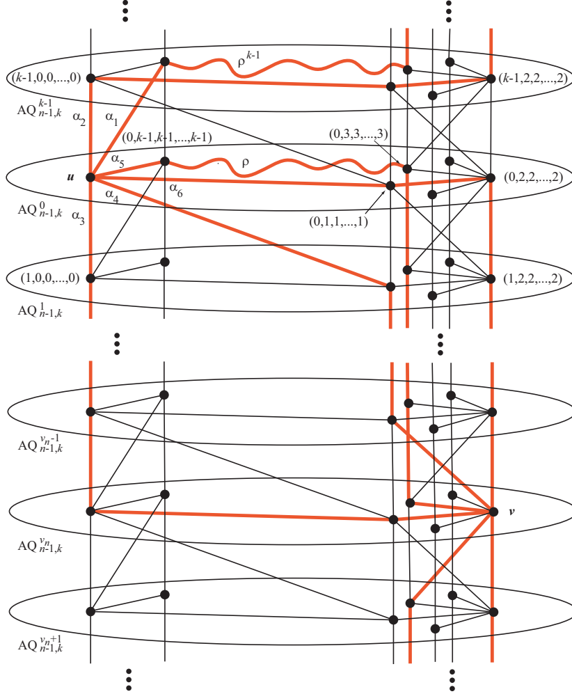
Figure 6. The paths in Sub-case 3.1.
