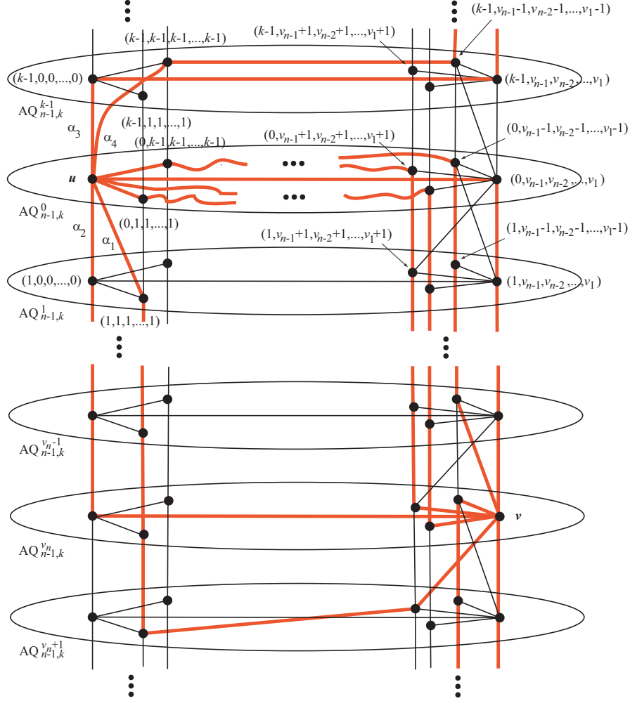
Figure 8. The paths in Sub-case 4.1.
