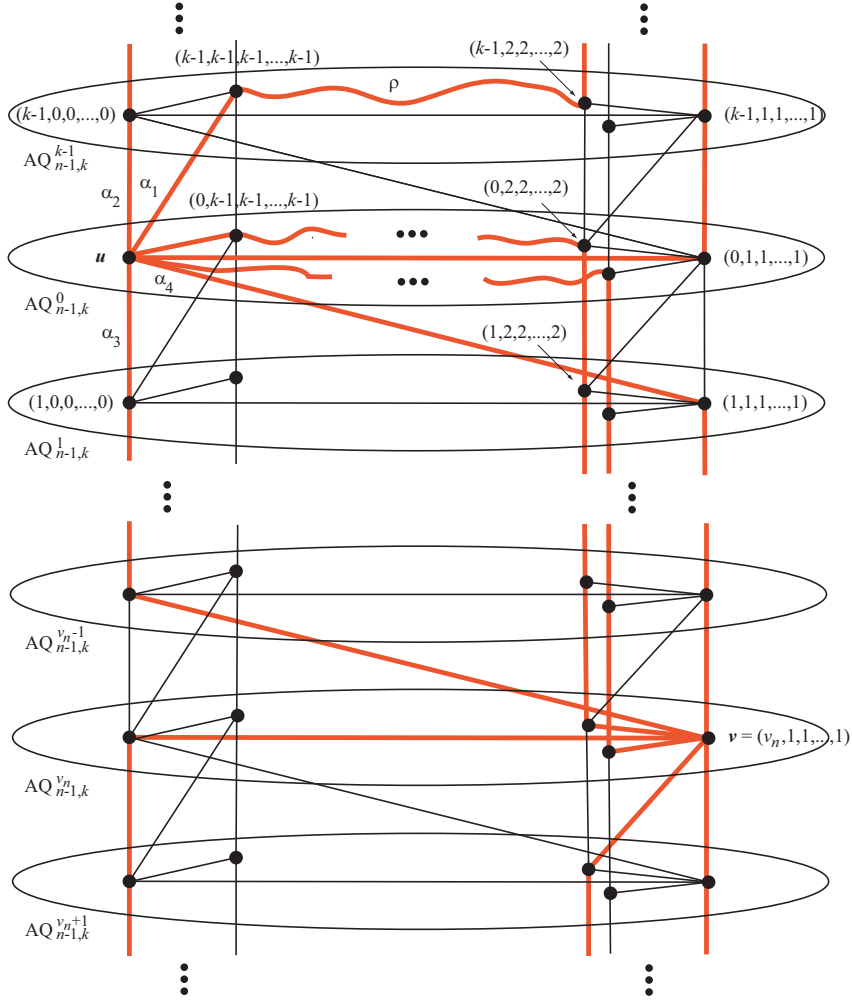
Figure 9. The paths in Sub-case 4.2.
