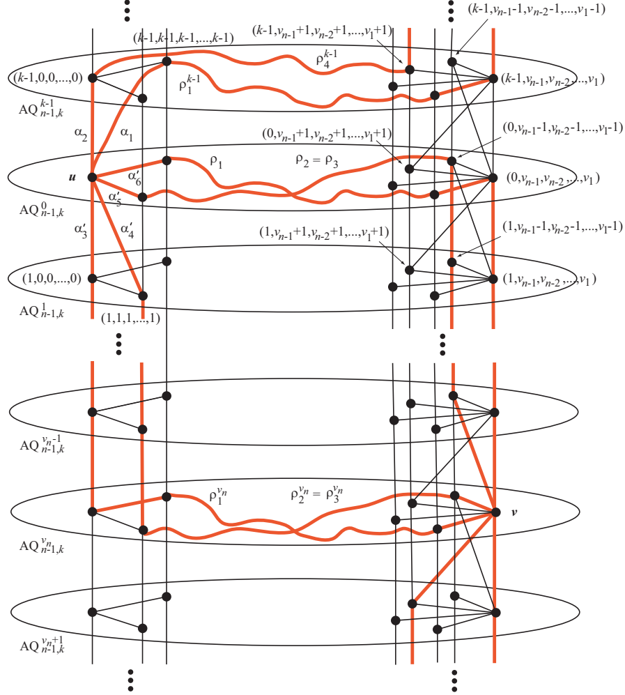
Figure 5. The amendments in Sub-case 2.3.
