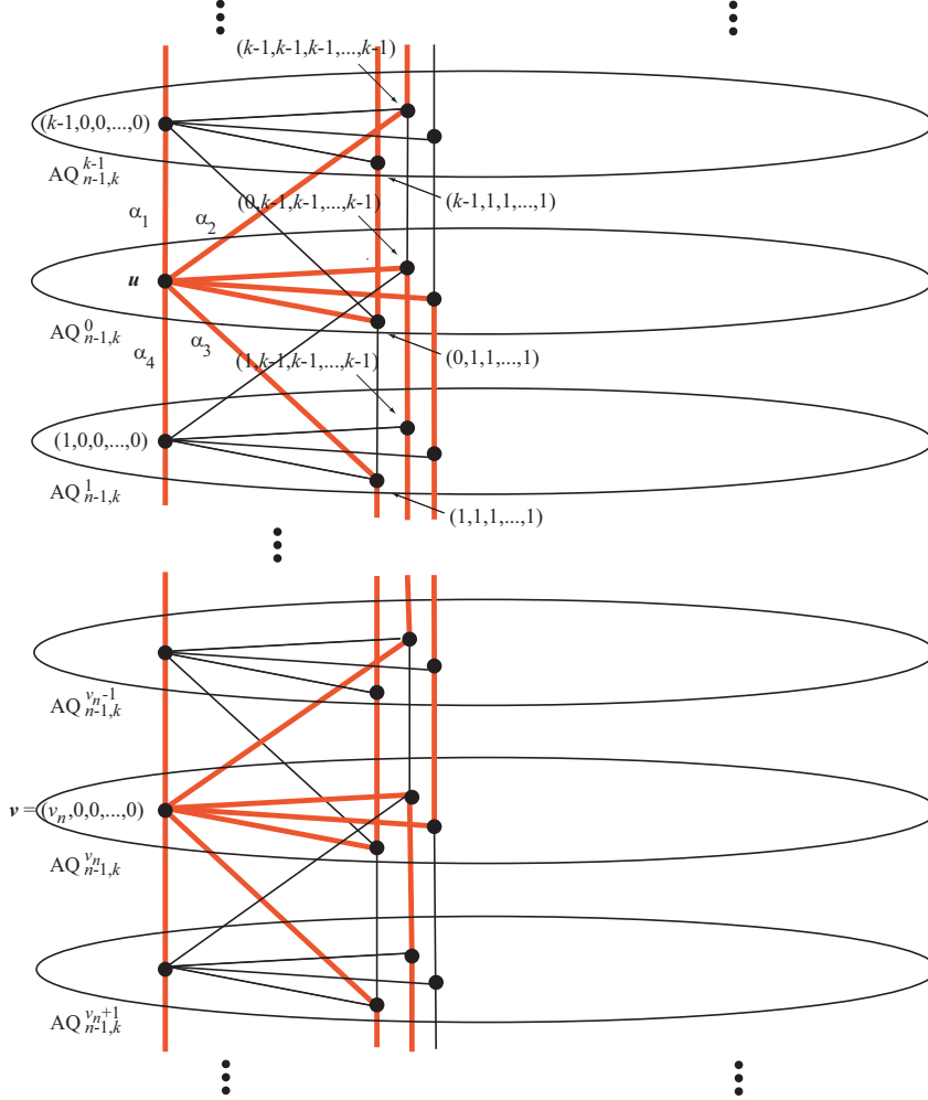
Figure 2. The 4n - 2 disjoint paths in Case 1.
