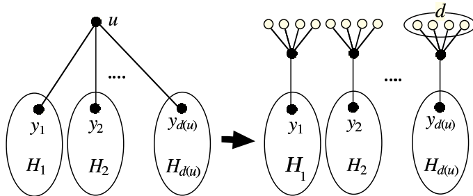
Fig. 1. From the tree H to the trees H'_i .
