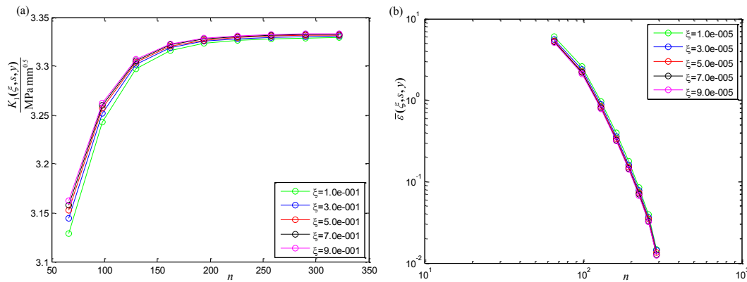
Figure 9. (a) Convergence and (b) convergence rate of % error in estimation of K_1 for through crack in finite plate
