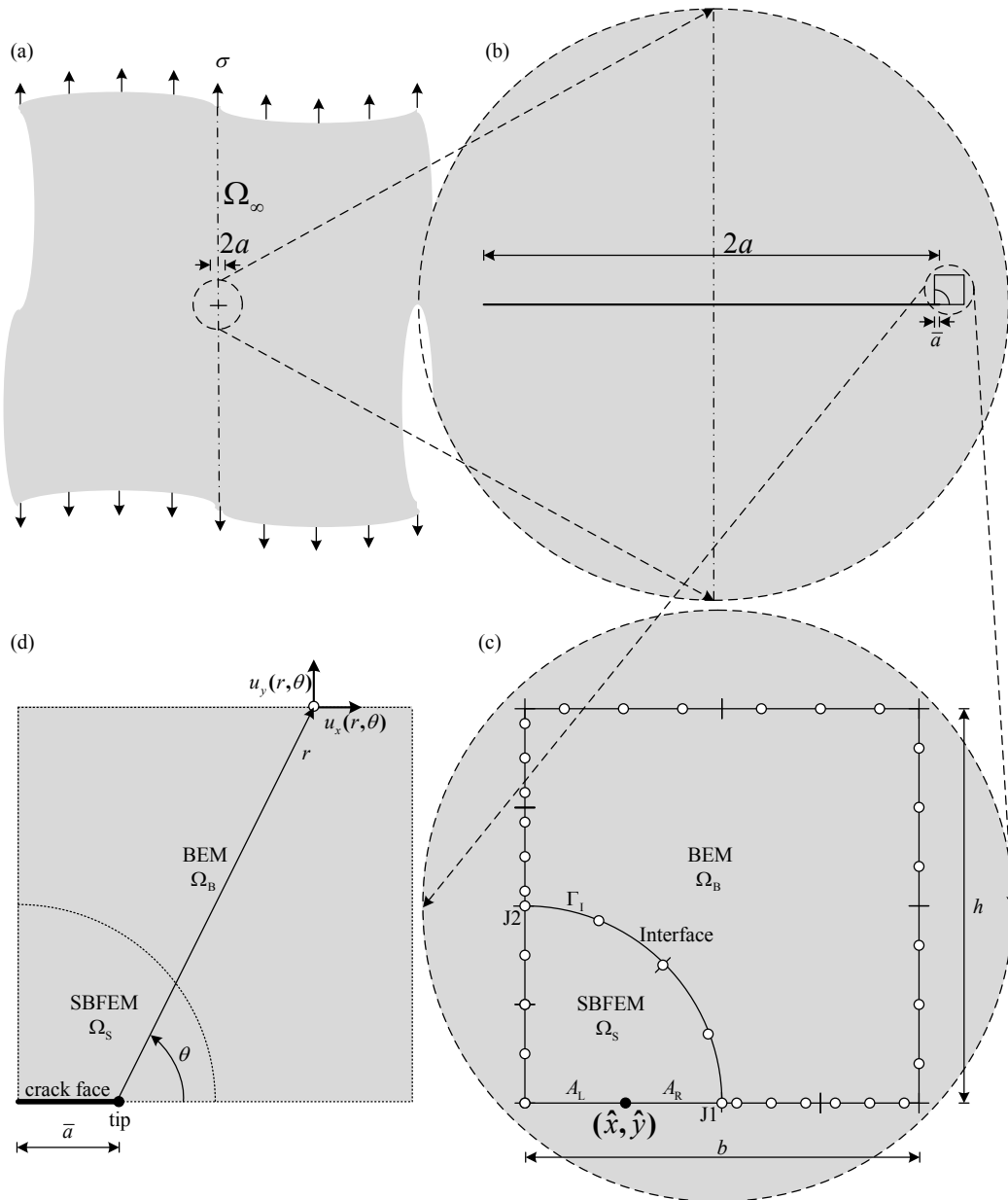
Figure 3. (a) Through crack in an infinite plate, (b) the section of the crack that is modelled, (c) the BE-SBFEM model of the immediate vicinity of the crack tip and (d) the Williams expansion coordinate system [17], used in the approximation of displacements u_x and u_y
