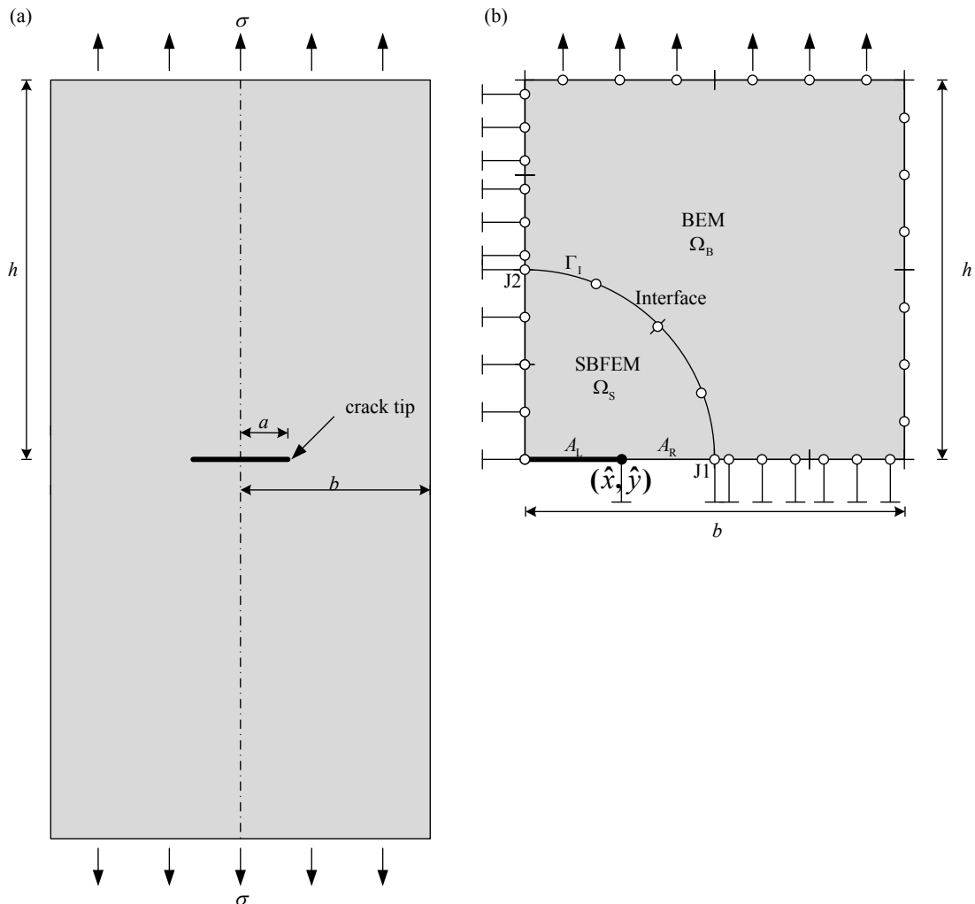
Figure 8. (a) The finite plate with through crack and (b) the BE-SBFEM model
